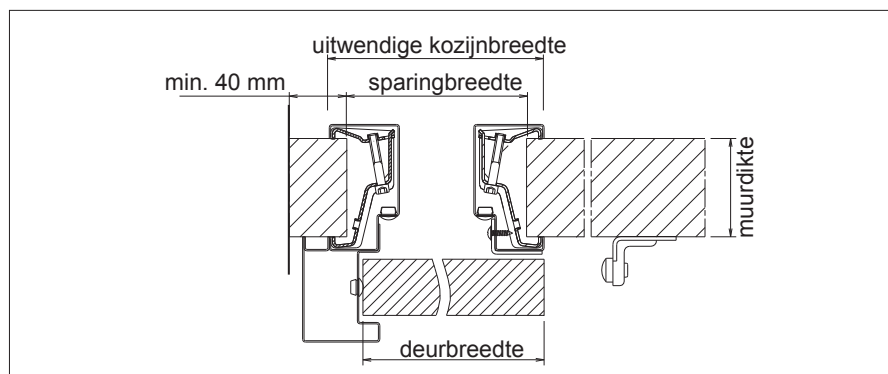
horizontale doorsnede model 1
