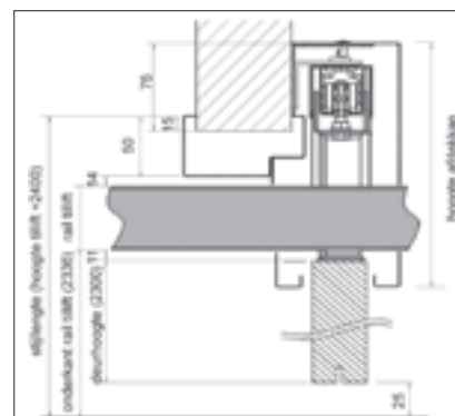
verticale doorsnede model 1
