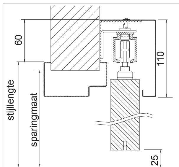
verticale doorsnede SVW Electric
